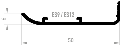
4575 COUVRE JOINT COURBÉ 50 mm Solape curvo 50 mm
