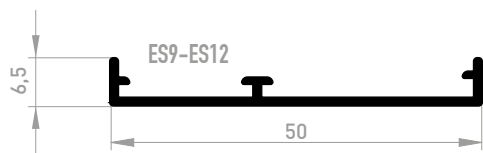
7196* COUVRE JOINT DROIT DE 50 mm GR. PLAST. Solape recto 50 mm gr.plast.
